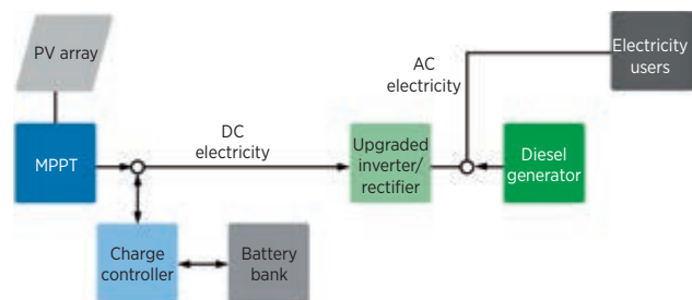
Figure B.2: Simplified diagram of a small hybrid system with storage and BoS equipment
